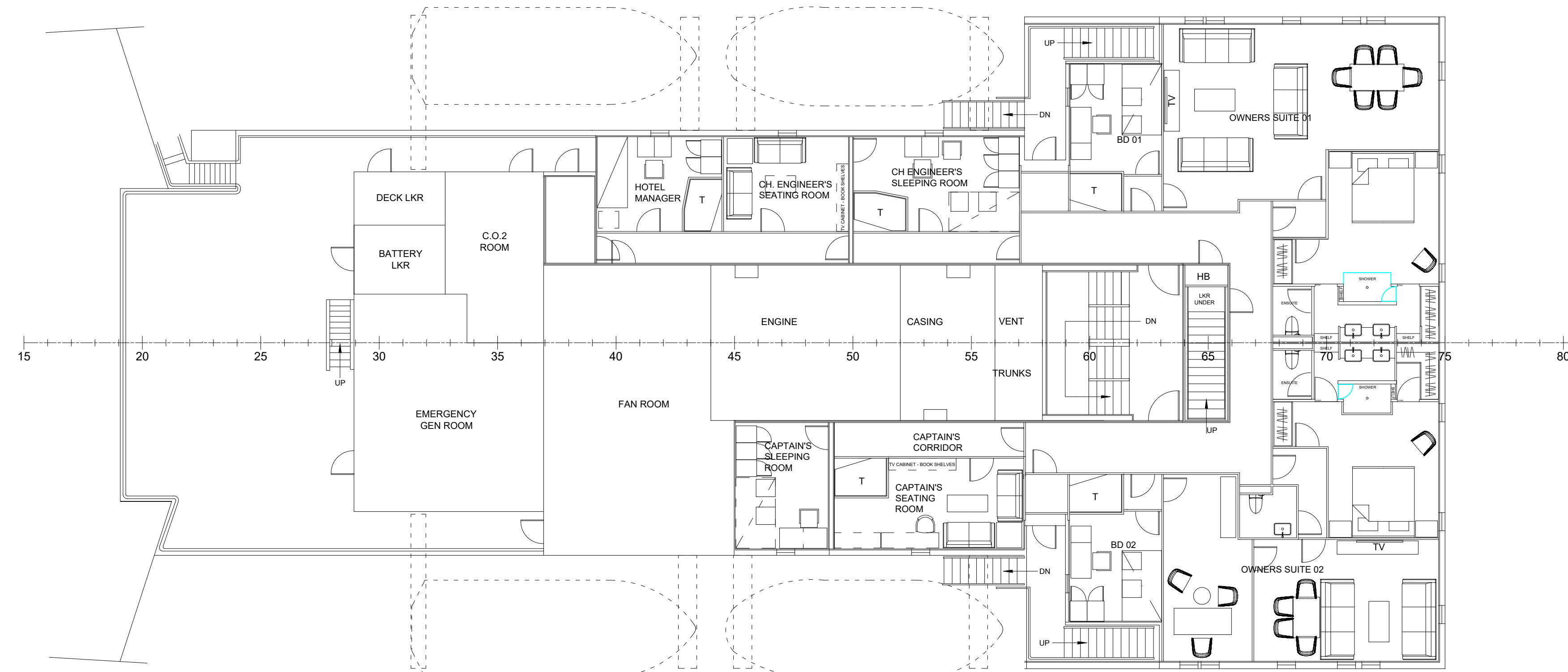
BOAT DECK
