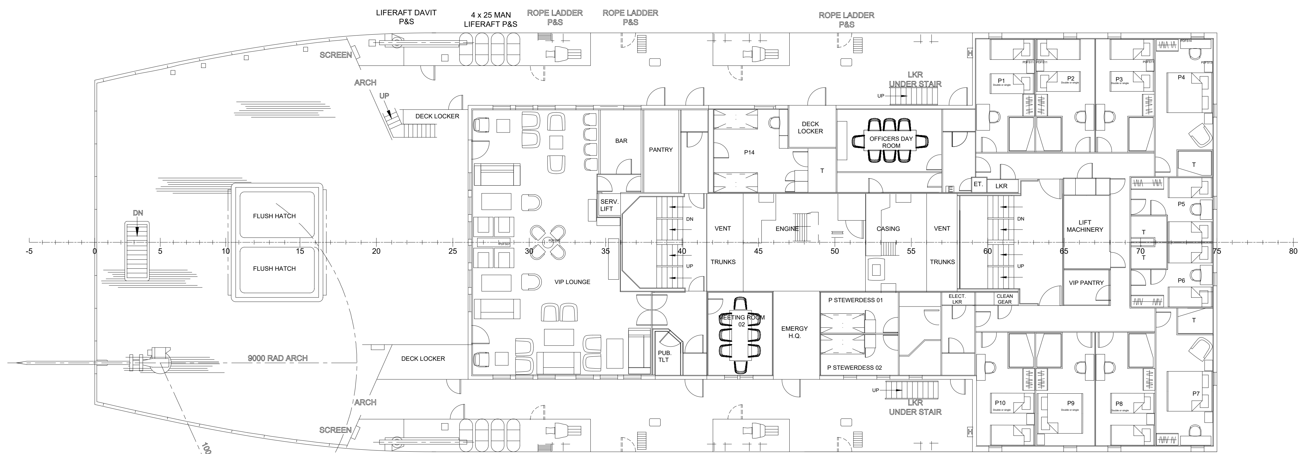
PROMENADE DECK
