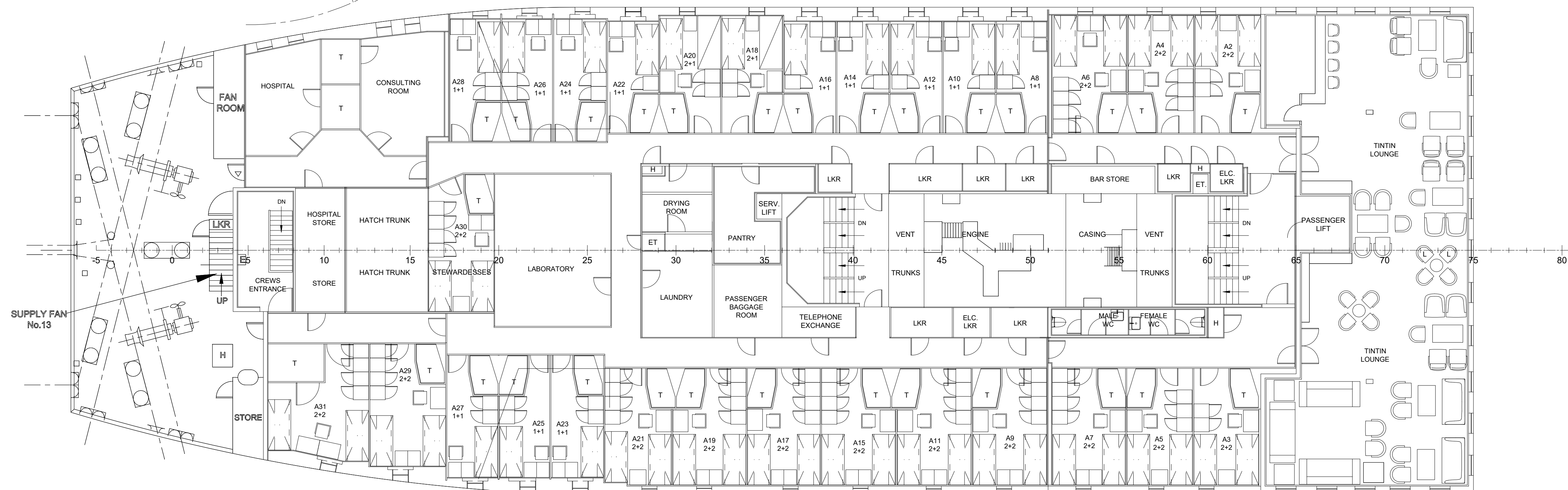
'A' DECK
