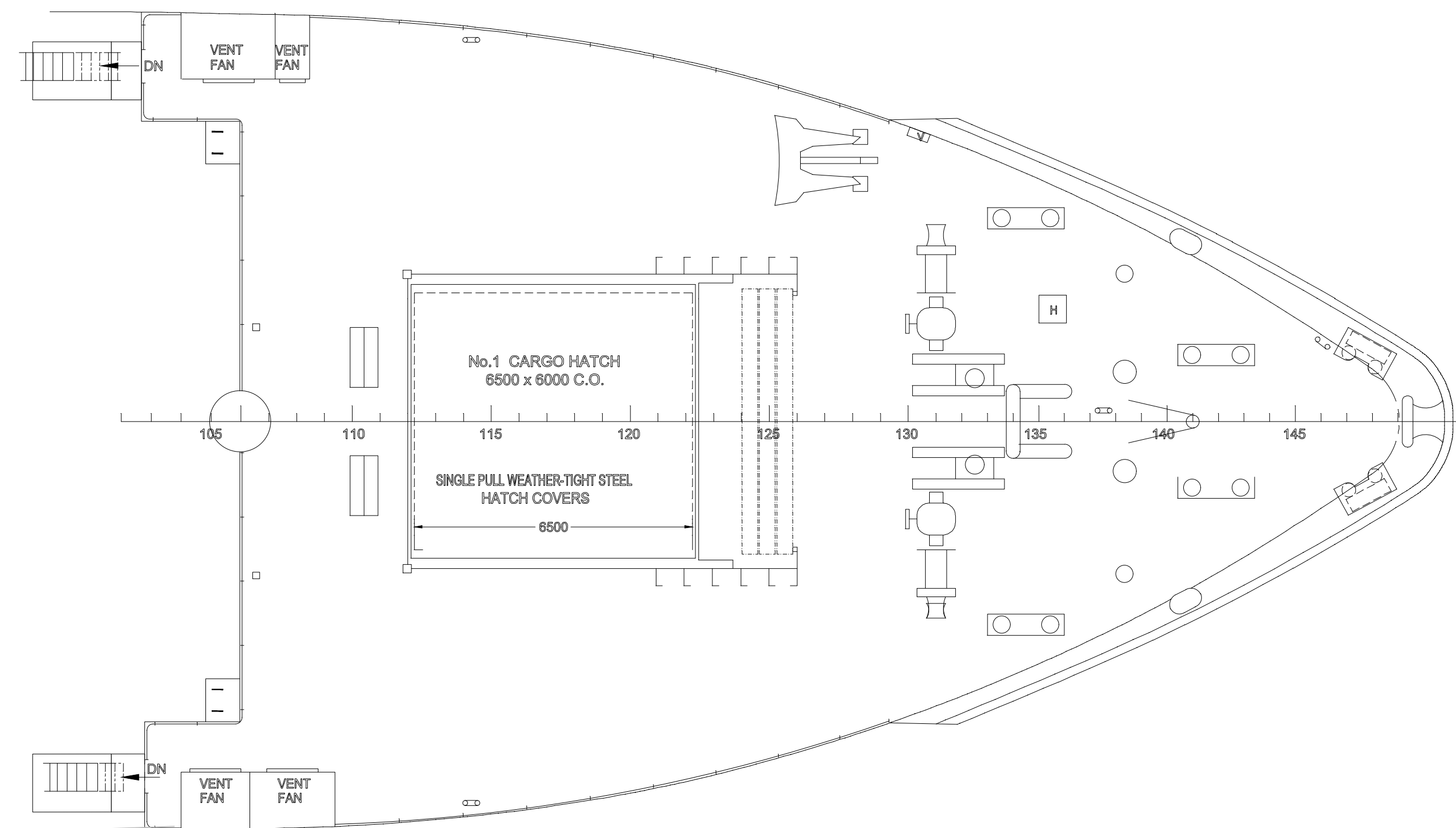
FORECASTLE DECK
